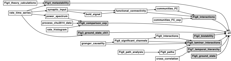
Figure 2. Visualization of a Snakemake workflow. The interdependencies between the scripts reproducing the figures in [12], visualized as a directed acyclic graph. The label of a node corresponds to the name of the script.
