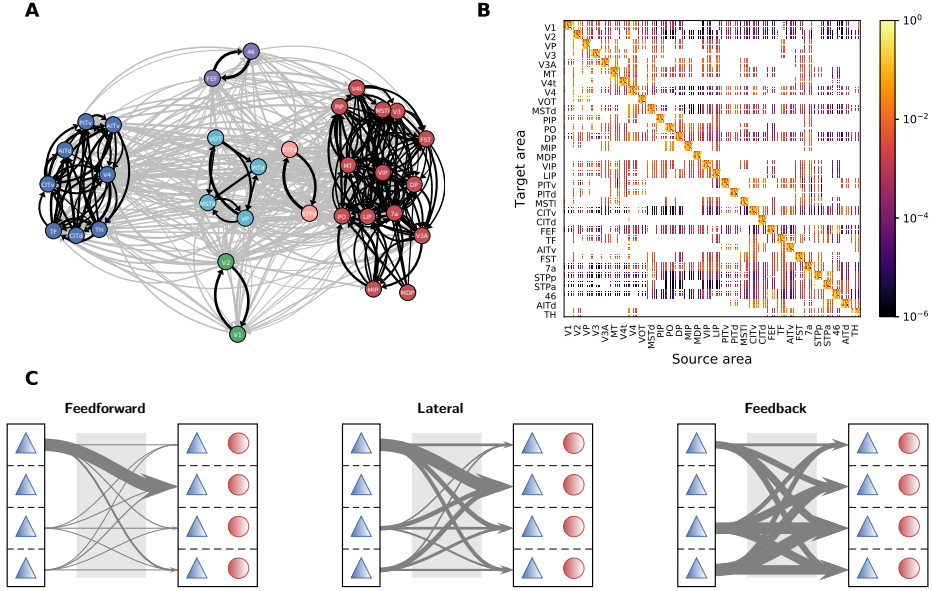
Figure 1. Overview of the connectivity of the multi-area model as determined from anatomical data and predictive connectomics. A Area-level connectivity. The weighted and directed graph of the number of outgoing synapses per neuron (out-degrees) between each pair of areas is clustered using the map equation method [20]. Green, early visual areas; dark blue, ventral stream areas; purple, frontal areas; red, dorsal stream areas; light red, superior temporal polysensory areas; light blue, mixed cluster. Black arrows show within-cluster connections, gray arrows between-cluster connections. B Population-level connection probabilities (the probability of at least one synapse between a pair of neurons from the given populations). C Hierarchically resolved average laminar patterns of the numbers of incoming synapses per neuron (in-degrees). Hierarchical relationships are defined based on fractions of supragranular labeled neurons ( SLN ) from retrograde tracing experiments [21]: feedforward, SLN > 0.65 ; lateral, 0.35 \leq SLN \leq 0.65 ; feedback, SLN < 0.35 . The connections emanate from excitatory neurons and are sent to both excitatory and inhibitory neurons. For further details see [11].
