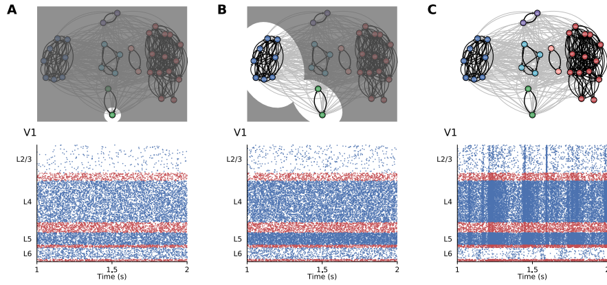
Figure 3. Simulating subsets of the multi-area model. Bottom panels, spiking activity of excitatory (blue) and inhibitory (red) neurons in all layers of area V1 where in A and B a subset of areas is replaced by Poisson processes. Top panels, sketches visualizing which areas were simulated (white spotlights); the colors therein correspond to different clusters: lower visual (green), ventral stream (dark blue), dorsal stream (red), superior temporal polysensory (light red), mixed cluster (light blue), and frontal (purple). If all areas besides V1 are replaced by Poisson processes ( A ), the activity displays no temporal structure. Simulating a subset of ten areas ( B ) slightly increases the activity but does not give rise to a temporal structure, either. Only the simulation of the full model ( C ) produces a clear temporal structure in the activity. Parameters identical to [12, Fig. 5].
