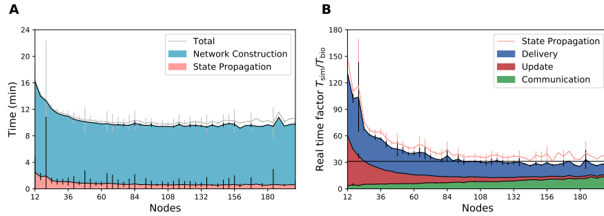
Figure 4. Strong scaling of the multi-area model. The contributions of different phases to the total simulation time and state propagation for 12 to 200 compute nodes for 1 s of biological time. Each data point consists of three random network realizations, with error bar showing the standard deviation of measurements. ( A ) The main contributions to the total time are network construction and state propagation. ( B ) The state propagation is dominated by three phases: the communication, update, and spike delivery phase. Adding more compute resources while keeping network size the same (strong scaling) decreases the latter two but increases the absolute and relative contribution of the communication phase. The combined contributions are minimized at a real-time factor of 31 (black horizontal line). Parameters identical to [12, Fig. 5].
